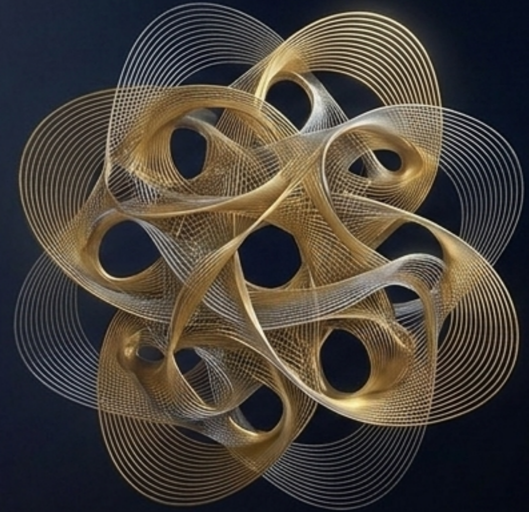
The Cosmic Landscape ( 10^{500} Vacua)
